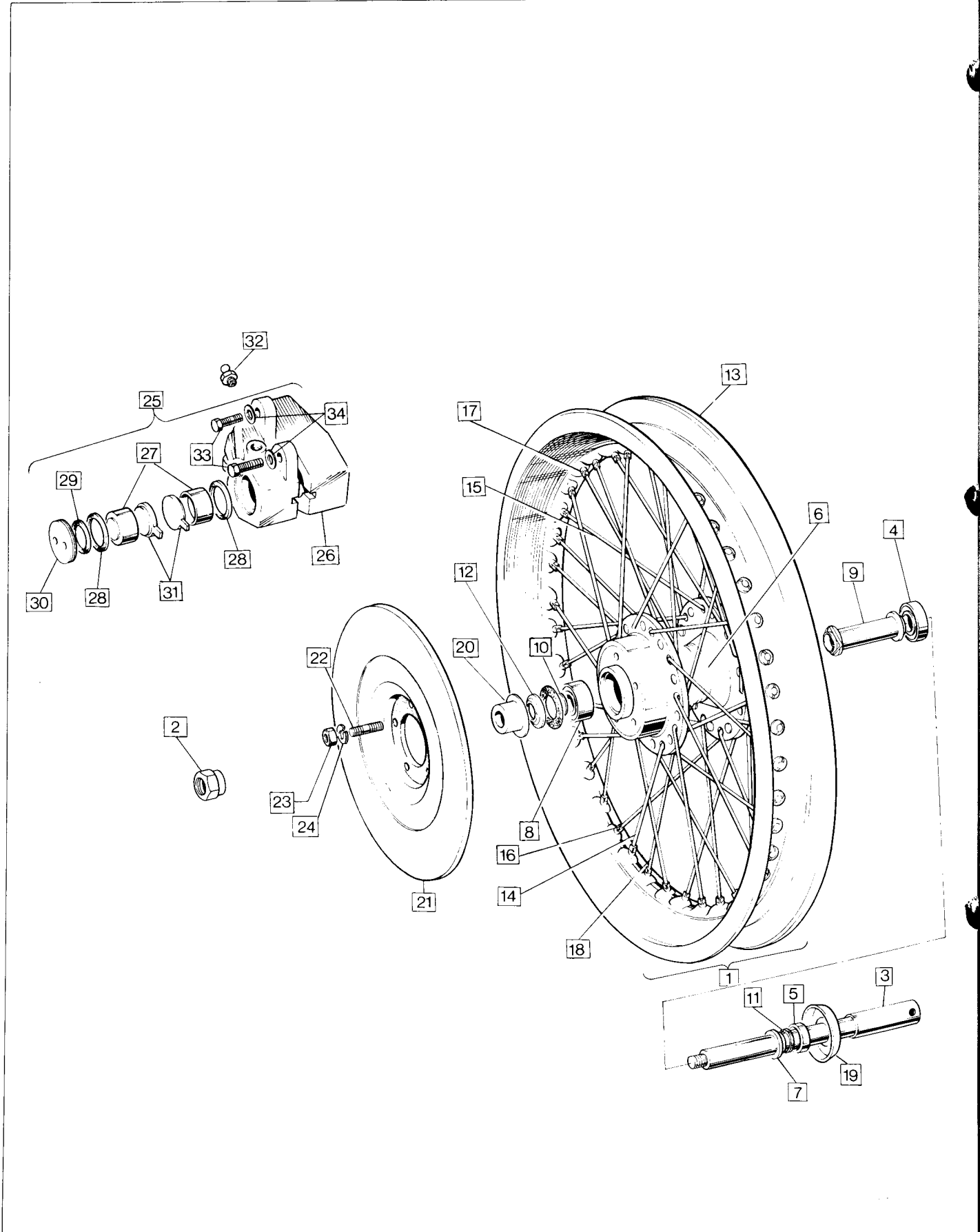
Front Wheel and Brake (Disc Type)
